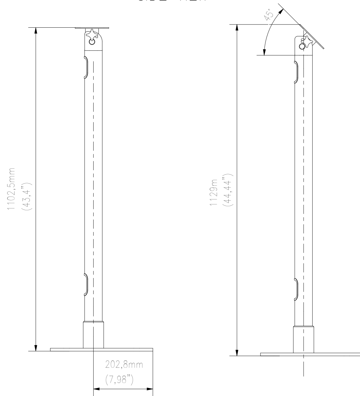
SIDE VIEW
