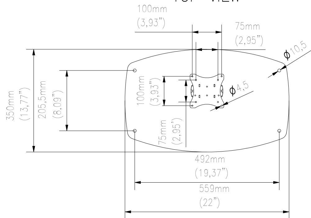
TOP VIEW
