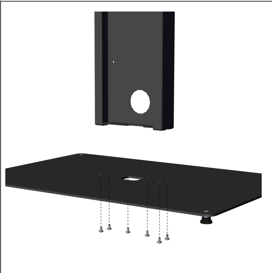
4. Connect the pillar to the bottom plate
